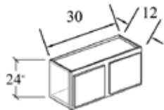
W3024
