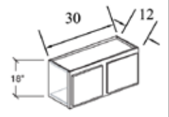
W3018
