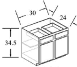
B30
